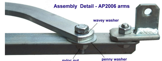
Assembly Detail - AP2006 arms
